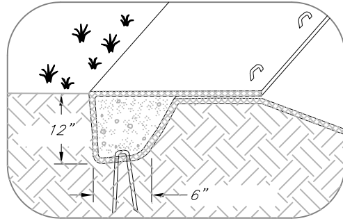
TERMINAL SLOPE AND CHANNEL ANCHOR TRENCH NTS
