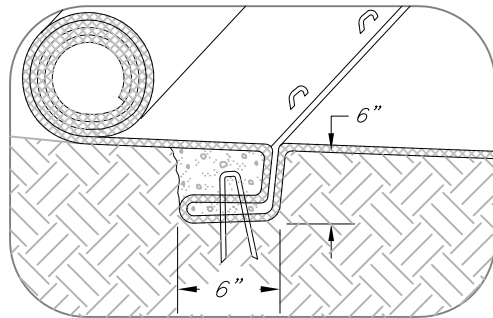
INTERMITTENT CHECK SLOT NTS
