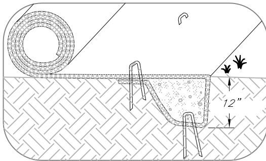
INITIAL CHANNEL ANCHOR TRENCH NTS
