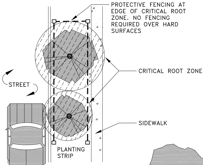
TYPICAL STREET TREE PROTECTION DETAIL
