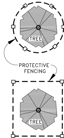
TYPICAL TREE PROTECTION (NO PAVED SURFACES)
