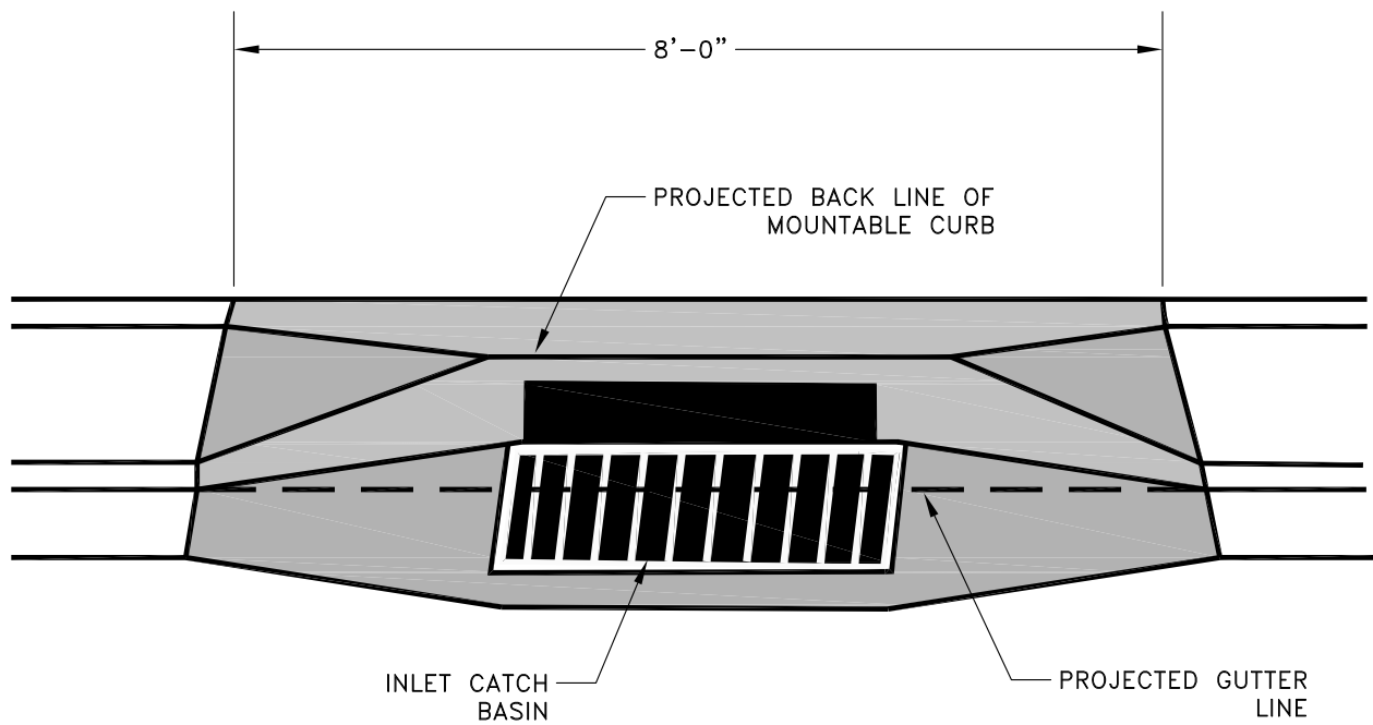
Front View
