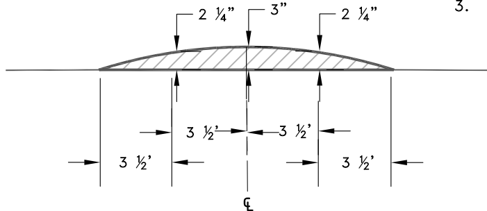
PARABOLIC CROWN SECTION A-A
