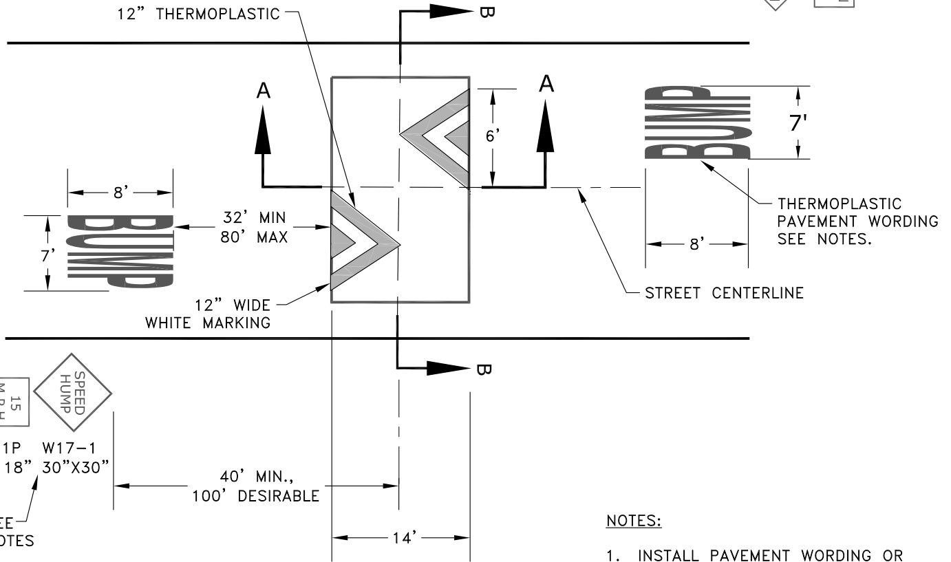
SPEED BUMP (TYPICAL)
